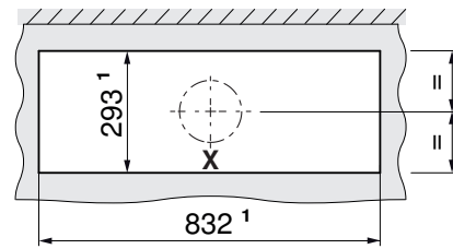
1 切面尺寸 1 Cut-out measurements
